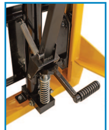
Foot pedal pump
