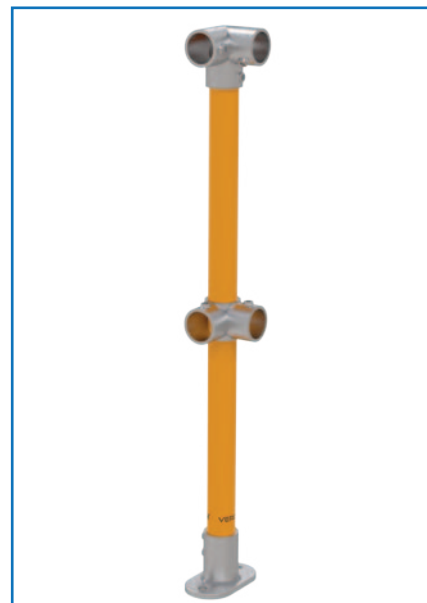
V7473 – Corner Post
