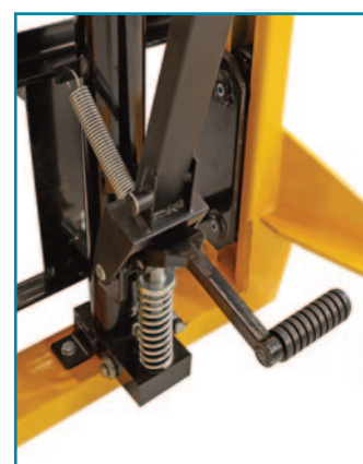
Foot pedal pump
